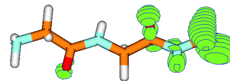
Hole density at t = 0
