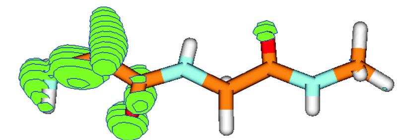
Hole density after 6 fs
