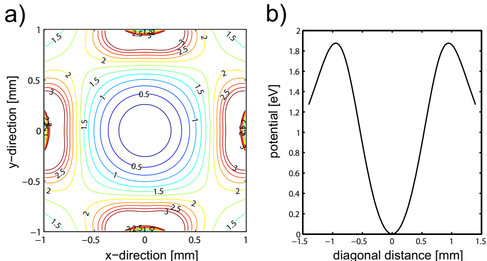
Figure 3. a) Simulation of the pseudo-potential in the x-y plane in the experimental zone for V = 408 V_{\text{pp}} . b) Cross-section through the potential shown in a) along the x = y direction yielding a radial trap frequency of \omega_{\text{rad}}/2\pi = 663 kHz and a trapping depth of approx. 1.9 eV.
