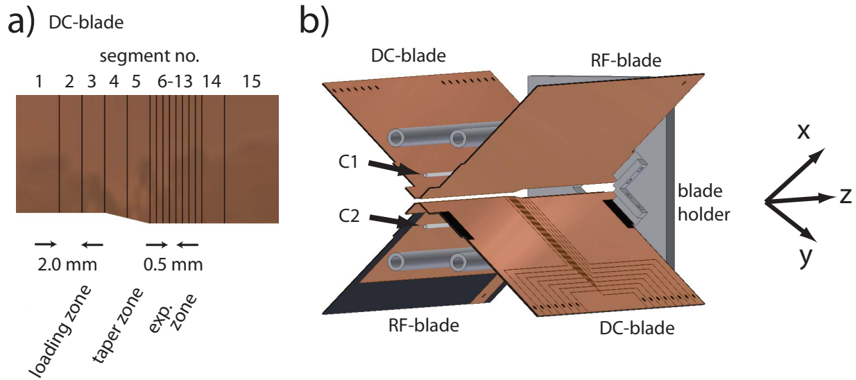
Figure 1. Electrode design. a) Close-up view of the blade design: The DC-blade segment width is 2 mm in the loading and taper zone, and 0.5 mm in the experimental zone. The trap consists of a 4 mm wide loading zone, a tapered intermediate zone, and a 2 mm wide experimental zone. b) Sketch of the assembled X-trap consisting of four blades, drawn with missing front blade holder for sake of clarity. Compensation electrodes C1 and C2 are parallel to the trap axis.
