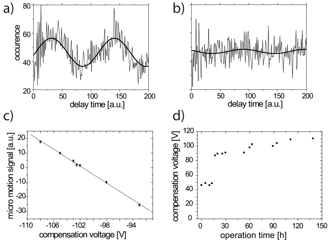
Figure 6. Histogram of photon count events for different values of micromotion compensation voltages: a) trace far from compensation with U_{C1} = 98 V fitted to a sine function. b) near to optimum compensation with U_{C1} = 102.5 V. c) The amplitude of a sinusoidal fit for different compensation voltages shows a linear dependence between the amplitude and applied compensation. Negative amplitudes correspond to a 180^\circ phase flip; this happens when the ion passes the RF null. A linear fit reveals the optimal value at U_{C1} = 101.6 V. With this data an optimal compensation is determined within an uncertainty of less than 0.3 V. The overall data collection time is less than 5 min. d) Optimum compensation voltage plotted versus the operation time of the oven. We attribute the long term drift of this voltage to an increasing calcium contamination on the trap electrodes in the experimental zone.
