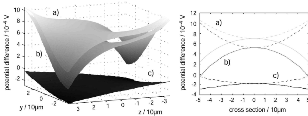
Fig. 14 a) Numeric result obtained by FEMLAB subtracted from the result of BEM [55], b) FEMLAB - CPO, c) CPO - BEM [55]. The left graph shows a 2D potential surface plot in the y - z plane. The right graph shows a line plot in the same plane in the direction of the two diagonal directions.
