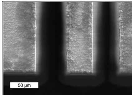
Fig. 2 Detail view on the trap chip, 5\mu\text{m} gold plated alumina of 125\mu\text{m} width cut by a fs-pulsed Ti:Sapphire laser. The scanning electron microscope picture shows several DC electrode segments of a single layer.
