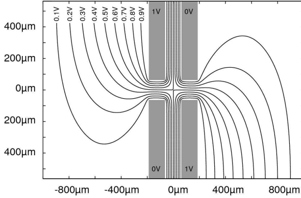
Fig. 3 Electric potential of the two-layer microstructure trap in radial direction ( yz cross section). Ions are confined by a pseudopotential on the x -axis. Here, the potential lines are normalized to a trap drive amplitude U_{rf} of 1V. In the central trapping region near the x -axis the electric potential may be approximated by a quadrupole potential as the radial harmonic pseudopotential for single ions.
