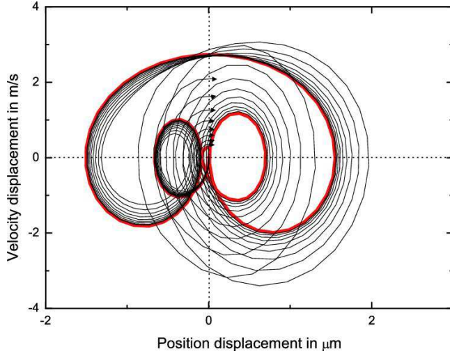
Fig. 9 Phase space trajectories in the frame co-moving with the potential minimum. The figure shows the trajectories pertaining to iterations 0, 10, ..., 100. At iteration 100, the ion arrives close to the origin. Note that the trajectory tends to be symmetrized by the optimization algorithm.
