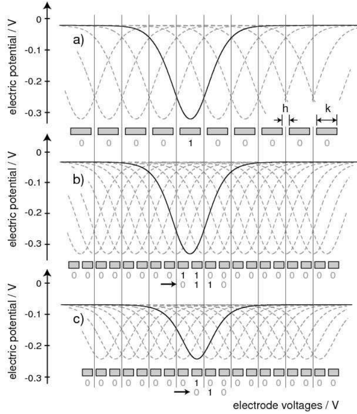
Fig. 5 Numerical calculation of the axial electric potentials \phi_{ax} , all cases (a) to (c) for the optimized radial slit width of g = 126 \mu\text{m} . a) DC segments with a width of k = 90 \mu\text{m} and gaps between axial electrodes of h = 30 \mu\text{m} result in a maximal d_2 coefficient. The potential of the adjacent electrode is plotted and shows only partial overlap (dashed gray). b) Optimized transport scheme: The DC electrodes are divided into equal parts with k = 45 \mu\text{m} and h = 15 \mu\text{m} . If both electrodes are at the same voltage of 1V, the potential is nearly identical to the optimized case (a). For transporting an ion, the potential minimum is shifted by changing the voltages from ..0/0/1/1/0/0.. \rightarrow ..0/0/0/1/1/0.. continuously. The axial potentials exhibit a large overlap which improves the transport of the ions. c) Simplified transport scheme: Axial potential for DC segments with k = 45 \mu\text{m} and h = 15 \mu\text{m} . Now, only a single segment is at 1 V. For transporting the voltages are changed from ..0/1/0/0/.. \rightarrow ..0/0/1/0/..
